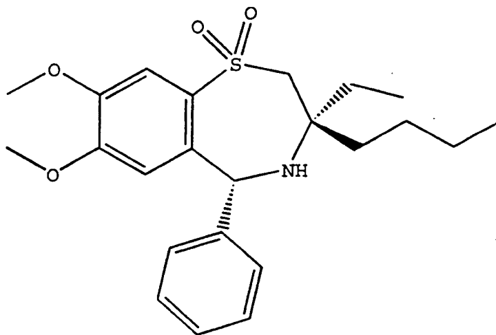
(3R,5R)-3-butyl-3-ethyl-2,3,4,5-tetrahydro-7,8-dimethoxy-5-phenyl-1,4-benzothiazepine 1,1-dioxide
